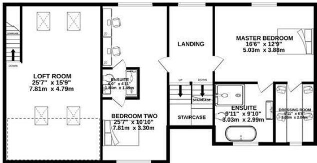
1ST FLOOR 1201 sq.ft. (111.6 sq.m.) approx.
